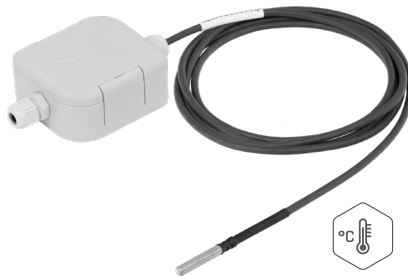
Temp-485-Pt100 Cable3 Probe temperature range: -50 to 200 °C, IP23 rating
