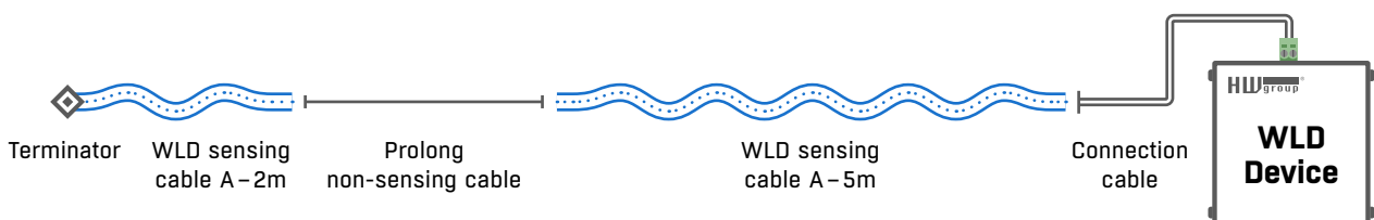
WLD A connection cable 2m 2m connection cable for connecting the WLD sensing cable with WLD zone input on any active device. WLD terminator included.
