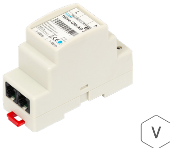
Sensor 230 V AC 1W-UNI Voltage range: 100-250 V AC
